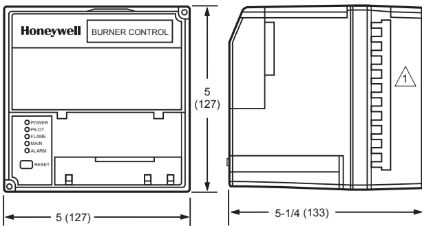
1 REMOVE ONLY FOR TERMINAL TEST ACCESS. M5003B
